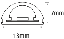
LED-NEON Dome, 4000K, 24 V
